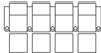
128" W x 38" D x 40" H 40/44/44/44-3440
